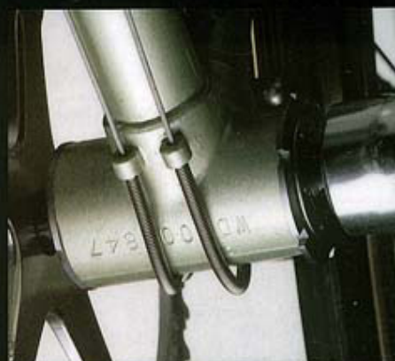
Under bottom bracket, cable guides and frame number
